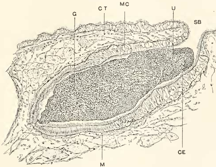
FIG. 3. Ostrca edulis , transverse section of left urinogenital cleft and spermiduct preserved during ejaculation. Both spermiduct ( G ) and the urinogenital cleft ( U ) are filled with ripe sperm. Camera lucida drawing \times 150 . Hæmatein-eosin.
